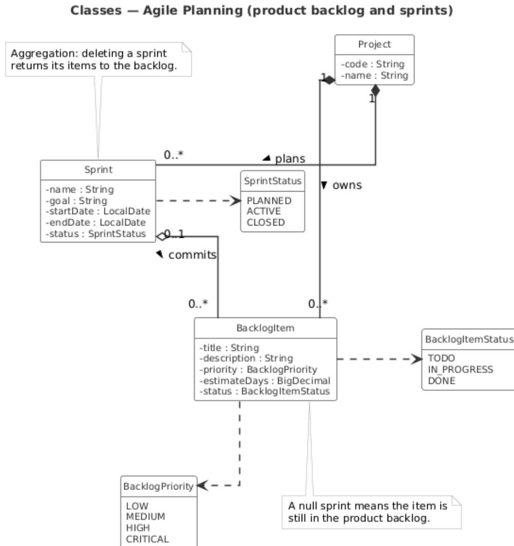
Figure 5.12: Class diagram — agile planning
