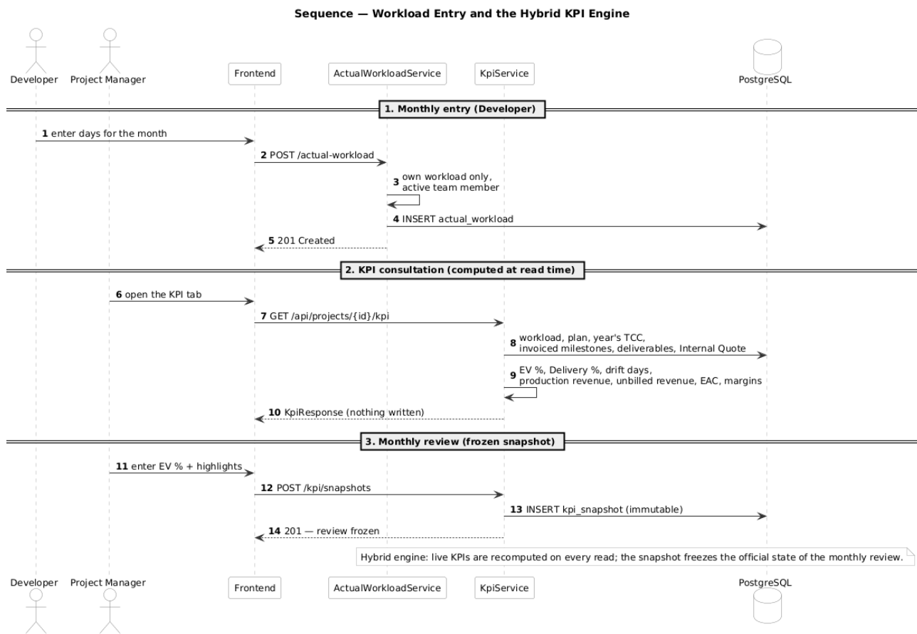
Figure 6.10: Sequence diagram — workload entry and indicator computation
